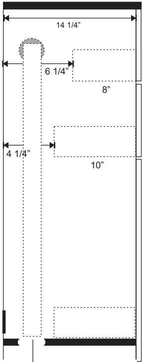
Basement installation
